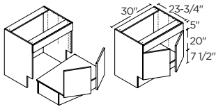
2 DOORS 30" | SB30FFRFADA
