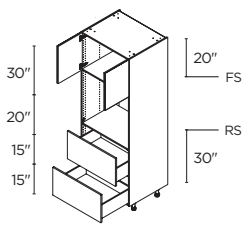
MICROWAVE 1 2 DOORS / 2 DRAWERS 30" | TM2D3084.5
