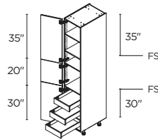
3 DOORS / 3 INNER DRAWERS 15" | T152489.5I3(L/R) 18" | T182489.5I3(L/R) 24" | T242489.5I3(L/R)
