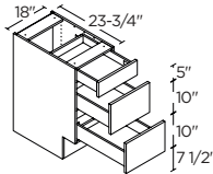
3 DRAWERS 18" | B3D18ADA
