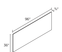
ISLAND PANEL 36" 5/8 x 96" | CP3696
