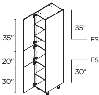
3 DOORS 15" | T152489.5(L/R) 18" | T182489.5(L/R) 24" | T242489.5(L/R)
