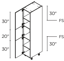
3 DOORS 15" | T152484.5(L/R) 18" | T182484.5(L/R) 24" | T242484.5(L/R)
