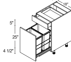
PULL-OUT / 1 DRAWER 18" | B18SWB Comes with 2 bins
