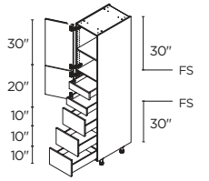
2 DOORS / 3 DRAWERS / 2 INNER DRAWERS 15" | T3DA152484.5I2(L/R) 18" | T3DA182484.5I2(L/R) 24" | T3DA242484.5I2(L/R)
