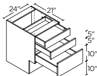
3 DRAWERS 24" | V3D24ADA
