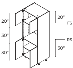
SINGLE OVEN 4 4 DOORS 30" | T03084.5
