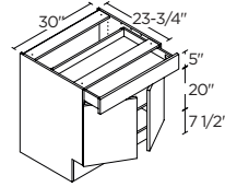
2 DOORS / 1 DRAWER 30" | B30ADA
