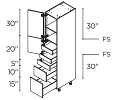
2 DOORS / 3 DRAWERS / 2 INNER DRAWERS 15" | T3D152484.5I2(L/R) 18" | T3D182484.5I2(L/R) 24" | T3D242484.5I2(L/R)
