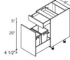
PULL-OUT / 1 DRAWER 18" | BP018 Comes with 2 bins
