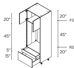
MICRO/WALL OVEN 2 2 DOORS / 2 DRAWERS 30" | TM02D3089.5
