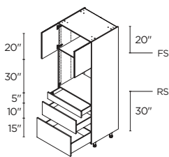
SINGLE OVEN 4 2 DOORS / 3 DRAWERS 30" | T03D3084.5
