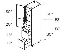
2 DOORS / 2 DRAWERS / 2 INNER DRAWERS 15" | T2D152484.5I2(L/R) 18" | T2D182484.5I2(L/R) 24" | T2D242484.5I2(L/R)
