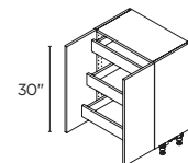
2 DOORS / 3 INNER DRAWERS 24" | B2414-2FHI3
