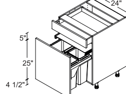
PULL-OUT / 1 DRAWER 24" | B24SWB Comes with 3 bins
