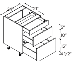
3 DRAWERS 24" | V3D24
