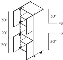
MICROWAVE 1 4 DOORS 30" | TM3084.5
