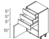
1 DOOR / 3 DRAWERS 15" | B1514C(L/R) 18" | B1814C(L/R)
