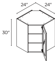
30" HIGH 1 GLASS DOOR* 24" | WAG2430(L/R)
