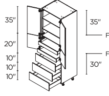
4 DOORS / 3 DRAWERS / 2 INNER DRAWERS 30" | T3DA302489.5I2
