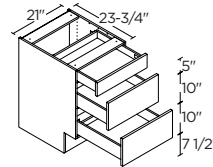
3 DRAWERS 21" | B3D21ADA
