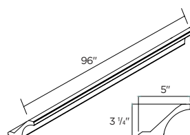
COVE PLAIN CROWN MOULDING With integrated cleat Available for Veneto & Barletta only 96 x 5 x 3 1/4" | CCMP96C
