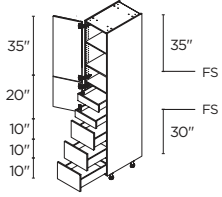
2 DOORS / 3 DRAWERS / 2 INNER DRAWERS 15" | T3DA152489.5I2(L/R) 18" | T3DA182489.5I2(L/R) 24" | T3DA242489.5I2(L/R)
