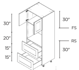
MICROWAVE 1 2 DOORS / 2 DRAWERS 30" | T02D3084.5
