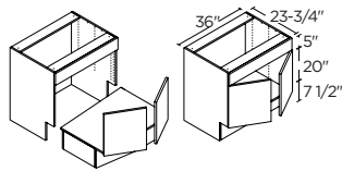
2 DOORS 36" | SB36FFRFADA
