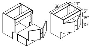
2 DOORS 36" | VS36FFRFADA
