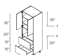
MICROWAVE 1 2 DOORS / 2 DRAWERS 30" | TM2D3089.5
