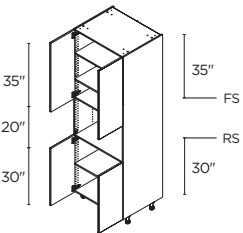
MICROWAVE 1 4 DOORS 30" | TM3089.5
