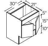
2 DOORS 30" | VS30ADA
