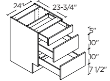
3 DRAWERS 24" | B3D24ADA
