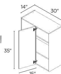
35" HIGH 1 DOOR 35" | WBL3035 35" | WBR3035
