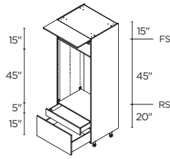
MICRO/WALL OVEN 2 1 LIFT-UP DOOR / 2 DRAWERS 30" | TM0L2D3084.5
