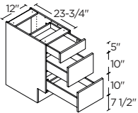
3 DRAWERS 12" | B3D12ADA
