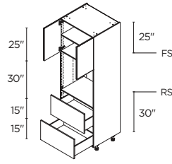
SINGLE OVEN 3 2 DOORS / 2 DRAWERS 30" | T02D3089.5
