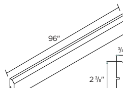
DECORATIVE MOULDING Available for Veneto & Barletta only 96 x 2 3/8 x 3/4" | DMC2.596
