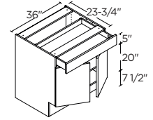
2 DOORS / 1 DRAWER 36" | B36ADA
