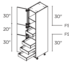
3 DOORS / 4 INNER DRAWERS 15" | T152484.5I4(L/R) 18" | T182484.5I4(L/R) 24" | T242484.5I4(L/R)
