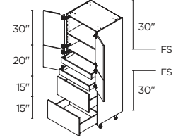
4 DOORS / 2 DRAWERS / 2 INNER DRAWERS 30" | T2D302484.5I2
