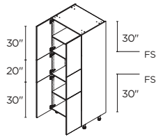
6 DOORS 30" | T302484.5
