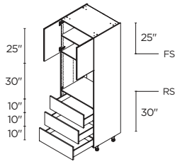
SINGLE OVEN 3 2 DOORS / 3 DRAWERS 30" | T03DA3089.5
