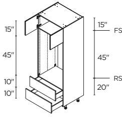
MICRO/WALL OVEN 2 2 DOORS / 2 DRAWERS 30" | TM02DA3084.5
