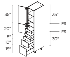
2 DOORS / 3 DRAWERS / 2 INNER DRAWERS 15" | T3D152489.5I2(L/R) 18" | T3D182489.5I2(L/R) 24" | T3D242489.5I2(L/R)
