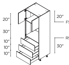
SINGLE OVEN 4 2 DOORS / 3 DRAWERS 30" | T03DA3084.5
