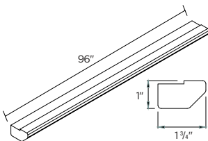
DECORATIVE LIGHT VALANCE MOULDING Not available for Sassari 96 x 1 x 1 3/4" | DLV96
