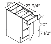
1 DOOR / 1 DRAWER 15" | B15ADA
