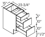
3 DRAWERS 15" | B3D15ADA
