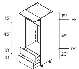
MICRO/WALL OVEN 2 1 LIFT-UP DOOR / 2 DRAWERS 30" | TM0L2DA3084.5
