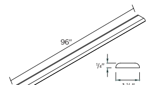
SCRIBE MOULDING Not available for Sassari 96 x 1/4 x 1 1/4" | SBM96
