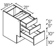
3 DRAWERS 18" | V3D18ADA
