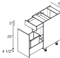
PULL-OUT / 1 DRAWER 15" | BP015 Comes with 1 bin
