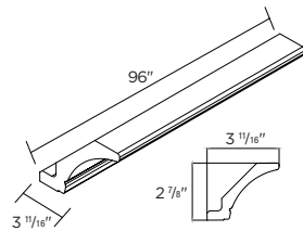
COVE CROWN MOULDING With integrated cleat Not available in Sassari 96 x 3 1/16 x 2 7/8" | CCM96C
