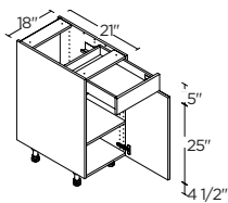
1 DOOR / 1 DRAWER 18" | V18(L/R)
