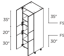
6 DOORS 30" | T302489.5
