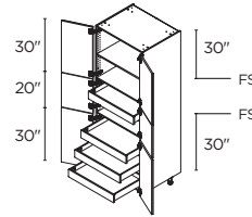
6 DOORS / 4 INNER DRAWERS 30" | T302484.5I4
