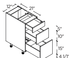
3 DRAWERS 12" | V3D12
