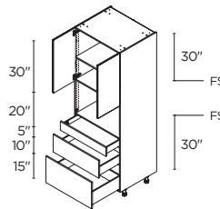
MICROWAVE 1 2 DOORS / 3 DRAWERS 30" | TM3D3084.5
