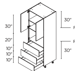
MICROWAVE 1 2 DOORS / 3 DRAWERS 30" | TM3DA3084.5
