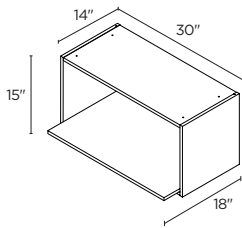
15" HIGH 30" | WMS3015
