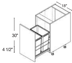
FULL HEIGHT DOOR 18" | B18FHSWB Comes with 2 bins
