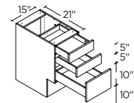
3 DRAWERS 15" | V3D15ADA
