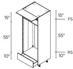
DOUBLE OVEN 3 1 LIFT-UP DOOR / 1 DRAWER 30" | TD0LA3084.5
