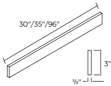
FILLER 3 x 5/8 x 30" | F330 3 x 5/8 x 35" | F335 3 x 5/8 x 96" | F396
