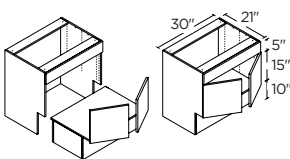
2 DOORS 30" | VS30FFRFADA
