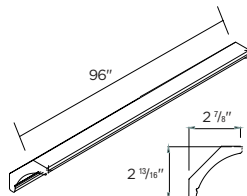
COVE CROWN MOULDING Without cleat Not available in Sassari 96 x 2 13/16 x 2 7/8" | CCM96NC
