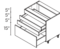
3 DRAWERS / 1 FIXED FRONT 36" | BCT4D36FF
