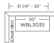
35" HIGH 1 DOOR 35" | WBL3035 35" | WBR3035
