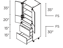
4 DOORS / 2 DRAWERS / 2 INNER DRAWERS 30" | T2D302489.5I2
