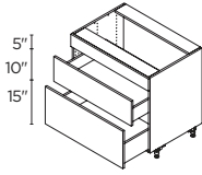
2 DRAWERS / 1 FIXED FRONT 36" | BCT3D36FF
