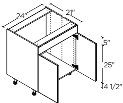
2 DOORS 24" | VS24
