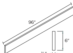
FILLER 6 x 5/8 x 96" | F696
