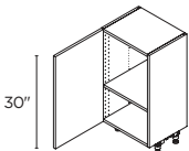
1 DOOR 9" | B914FH(L/R) 12" | B1214FH(L/R) 15" | B1514FH(L/R) 18" | B1814FH(L/R) 21" | B2114FH(L/R) 24" | B2414FH(L/R)
