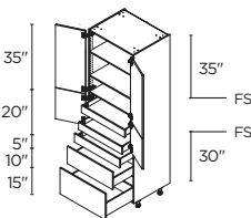
4 DOORS / 3 DRAWERS / 2 INNER DRAWERS 30" | T3D302489.5I2
