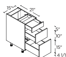
3 DRAWERS 15" | V3D15
