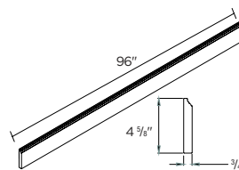
FURNITURE BASE MOULDING Available for Veneto & Barletta only 96 x 3/4 x 4 5/8" | FBM96
