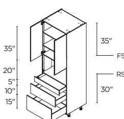
MICROWAVE 1 2 DOORS / 3 DRAWERS 30" | TM3D3089.5
