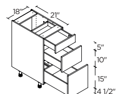
3 DRAWERS 18" | V3D18
