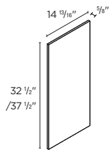
WALL CABINET COVER PANEL 14 13/16" 5/8 x 32 1/2" | CP1432 5/8 x 37 1/2" | CP1437
