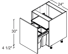
FULL HEIGHT DOOR 24" | B24FHSWB Comes with 3 bins
