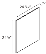
BASE CABINET COVER PANEL 24 13/16" 5/8 x 34 1/2" | CP2434
