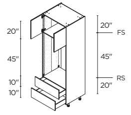
MICRO/WALL OVEN 2 2 DOORS / 2 DRAWERS 30" | TM02DA3089.5
