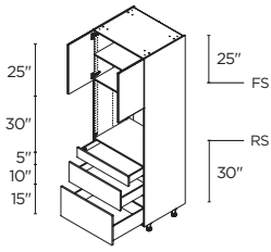
SINGLE OVEN 3 2 DOORS / 3 DRAWERS 30" | T03D3089.5
