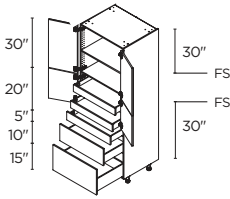
4 DOORS / 3 DRAWERS / 2 INNER DRAWERS 30" | T3D302484.5I2
