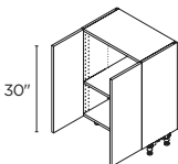
2 DOORS 24" | B2414-2FH 27" | B2714FH 30" | B3014FH 33" | B3314FH 36" | B3614FH
